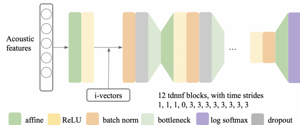
Figure 1: The TDNNF-architecture.
